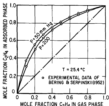
Fig. 9. Prediction of equilibrium gas- and adsorbed-phase compositions by ideal solution theory, ethylene-carbon dioxide mixtures
