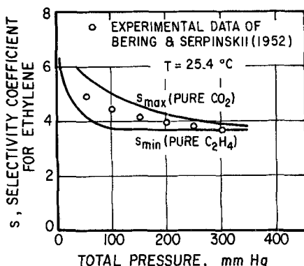
Fig. 10. Prediction of ideal solution theory: selectivity coefficient varies with vapor composition and total pressure.
